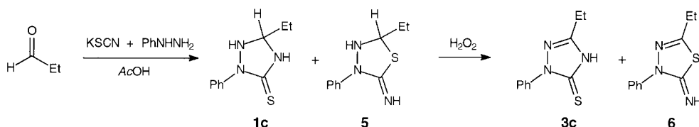
Scheme 2. Synthesis of the 1,2,4-Triazolidine-3-thione and 1,3,4-Thiadiazolidine-2-imine Derivatives 1c and 5 , Respectively, and Their Oxidation Products 3c and 6 , Respectively.
